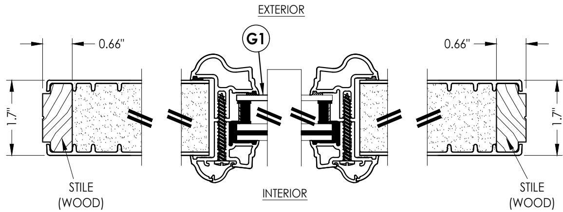
1 3 HORIZONTAL CROSS SECTION
