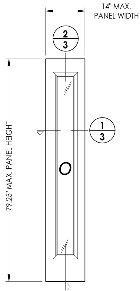
50 SIDELITE PANEL
